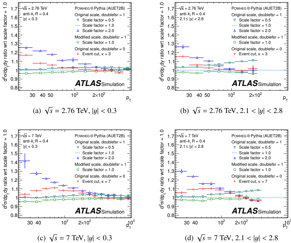
Figure 2.13: Comparison of the predictions for the inclusive jet cross-section from POWHEG for different matching scale choices in a ratio to the prediction using the nominal original scale with \text{doublefsr}=1 , separately for two centre-of-mass energies and two rapidity bins. The used parton shower Monte Carlo simulation is PYTHIA with the tune AUET2B. The jet algorithm is anti- k_t with a radius parameter of R = 0.4 . Also shown is the prediction using an event cut to suppress spikes in the final distributions [2]. Results for R = 0.6 are very similar.
