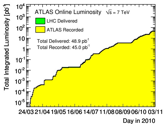
Figure 6.2: Total integrated delivered and recorded luminosity of proton-proton collision data in 2010 as function of time.
