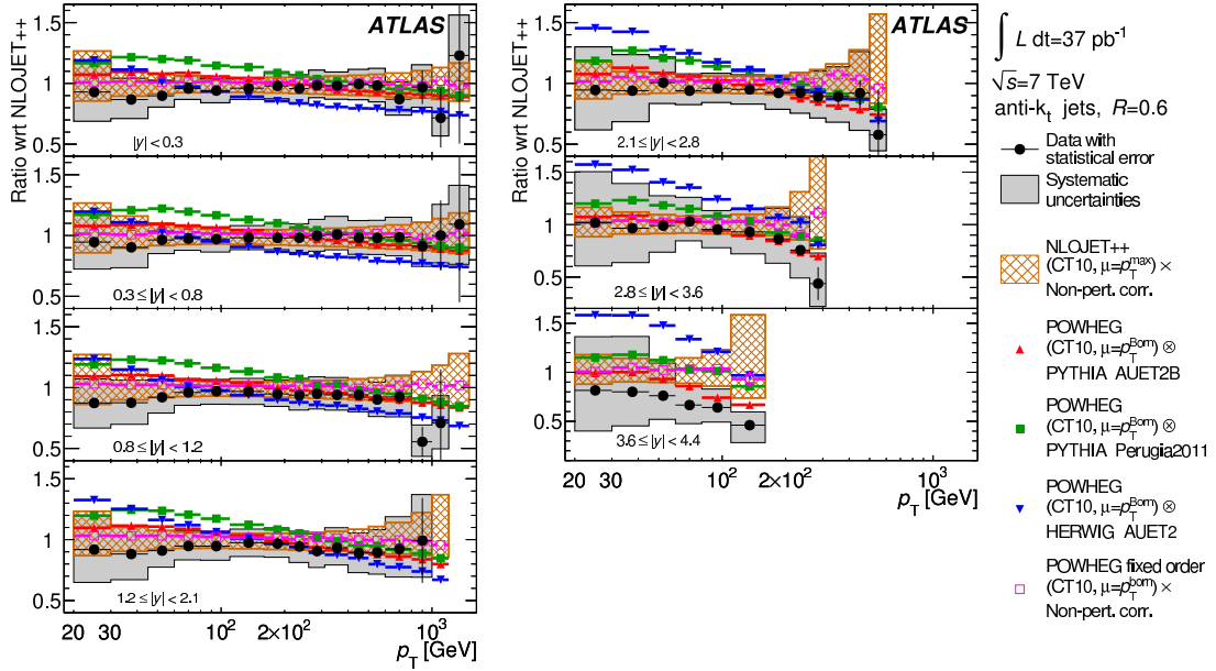
Figure 6.13: Ratio of the measured double-differential inclusive jet cross-section at \sqrt{s} = 7 \text{ TeV} for anti- k_t jets with a radius parameter of R = 0.6 with respect to the theoretical predictions from a perturbative QCD calculation at NLO precision using NLOJET++ with the CT 10 PDF set, corrected for non-perturbative effects. The ratio is shown as function of p_T separately for seven different bins of rapidity. The shaded and hatched area indicate the experimental and theoretical systematic uncertainties, respectively. Also shown are theoretical predictions obtained with the PowHEG generator, interfaced to the parton shower simulators PYTHIA using the tunes AUET 2B and PERUGIA 2011, and HERWIG using the tune AUET 2, and PowHEG using a fixed-order calculation at NLO precision with non-perturbative corrections applied. Only the statistical uncertainty is shown on the PowHEG prediction. Statistically insignificant data points at large p_T are omitted. The uncertainty due to the luminosity measurement of 3.4% is not shown [2].
