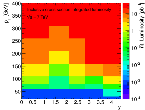
Figure 6.4: Total integrated luminosity after the trigger selection in each (y, p_{\text{T}}) bin of the inclusive jet cross-section measurement at \sqrt{s} = 7 TeV.
