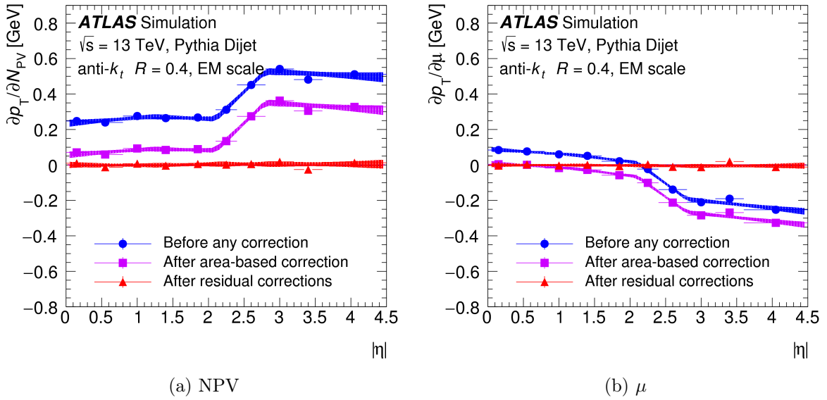
Figure 5.4: The dependence of EM-scale jet p_T on (a) NPV averaged over \mu and (b) \mu averaged over NPV as a function of |\eta| for p_T^{truth} = 25 GeV is shown. The dependence on \eta is shown prior to pile-up corrections (blue circle), after the area-based correction (violet square), and after the residual correction (red triangle) are applied. The shaded bands represent the 68% confidence intervals of the linear fits in 4 regions of |\eta| . Taken from [66].
