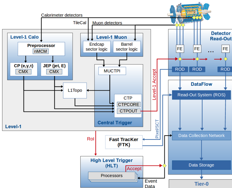
Figure 6.1: The components of the ATLAS trigger and data acquisition system are shown, and referred to in the text. Taken from [68]
