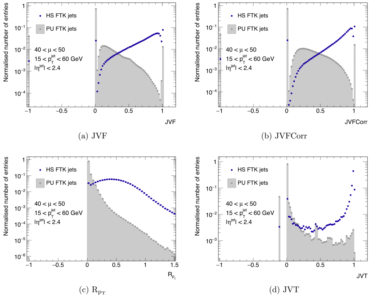
Figure 11.4: Variable distributions for hard scatter jets (blue) are contrasted against those for pile-up jets (grey), for 40 < \mu < 50 and jets with 15 < \text{jet } p_T < 60 GeV, jet |\eta| < 2.4 . The separation in the distributions offers a way of discriminating between hard scatter and pile-up jets. More distinct distributions will lead to a higher hard scatter jet acceptance rate with an accompanying lower pile-up jet acceptance rate.
