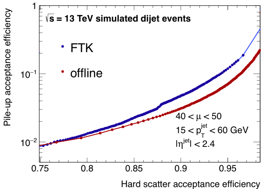
Figure 11.9: The acceptance efficiency of hard scatter jets versus pile-up jets is shown for (a) JVFCorr and (b) Rp T for FTK (blue) and offline jets (red). Only jets with 15 < \text{jet } p_T < 60 \text{ GeV} and \text{jet } |\eta| < 2.4 are included. At equal true positive efficiencies of 92%, the accompanying fake rate for JVT is 3% higher for FTK jets compared to offline jets.
