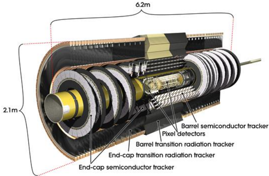
Figure 5.2: The ATLAS inner detector is a tracking system that makes use of pixel and silicon microstrip trackers and straw tubes of a transition radiation tracker in order to measure momenta and vertices of charged particle tracks with high precision. Taken from [50].
