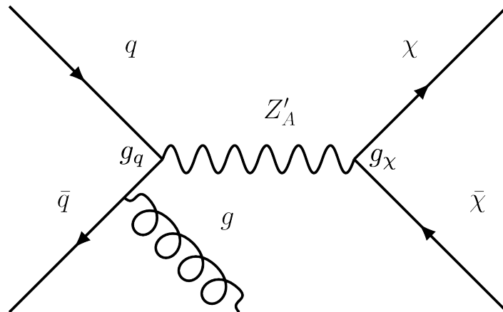
Figure 3.3: An example signature for E_T^{\text{miss}} +associated SM particle searches conducted at colliders, in which dark matter particles are pair-produced along with an initial state radiation gluon. The particle mediating the interaction is assumed to be an axial-vector boson, Z'_A . The dark matter particles are expected to leave no measurable trace in the detector. The process can however be identified by the missing transverse energy, E_T^{\text{miss}} , counteracting the transverse energy of the associated jet.
