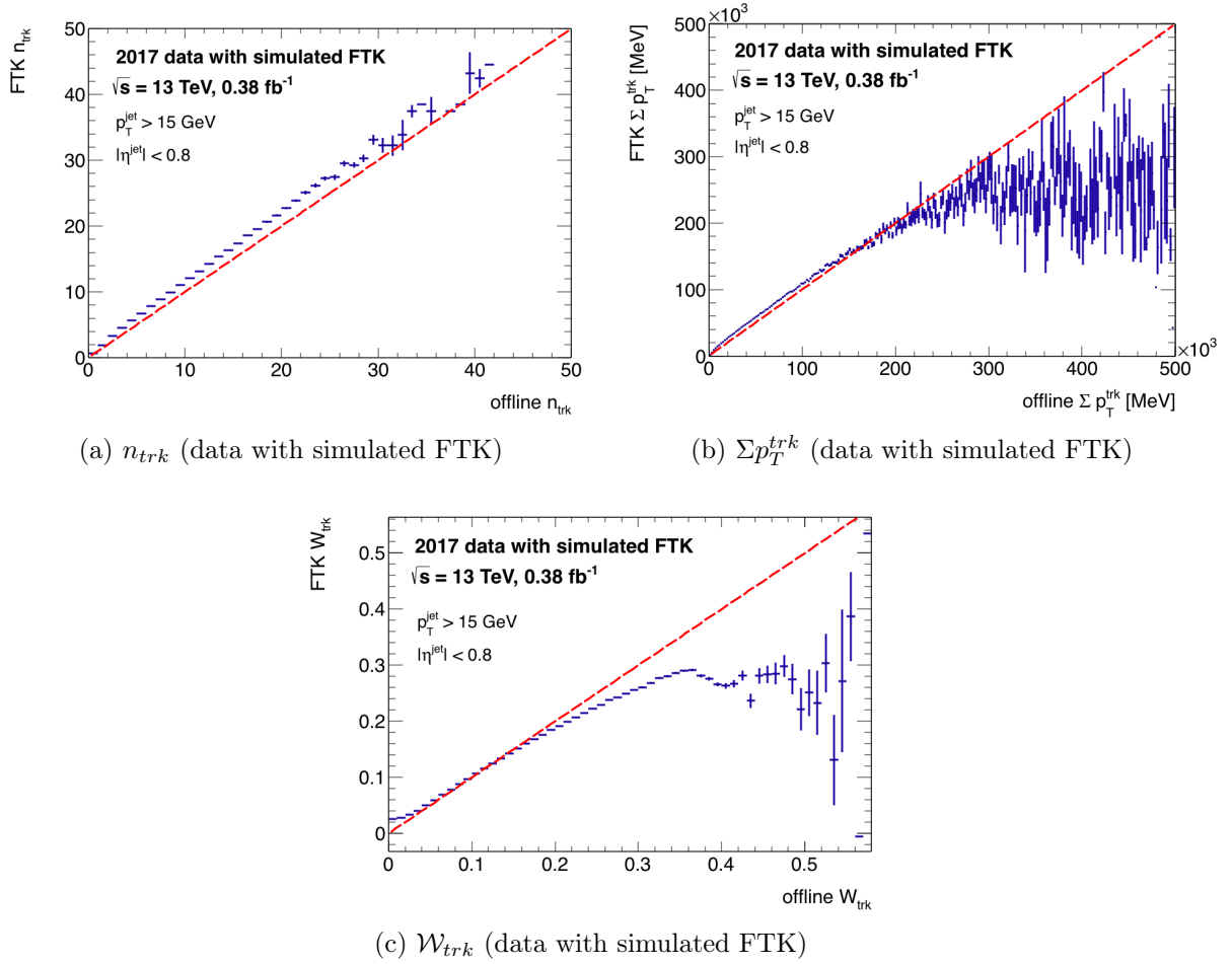
Figure 10.6: A comparison between FTK and offline jets is shown for three jet track attributes: n_{trk} , \Sigma p_T^{trk} and W_{trk} , for jets with p_T > 15 \text{ GeV} and |\eta| < 0.8 and tracks with p_T > 1 \text{ GeV} . 2017 data is reprocessed from digitised data with a simulated FTK system. FTK jets are reconstructed in the HLT jet trigger.
