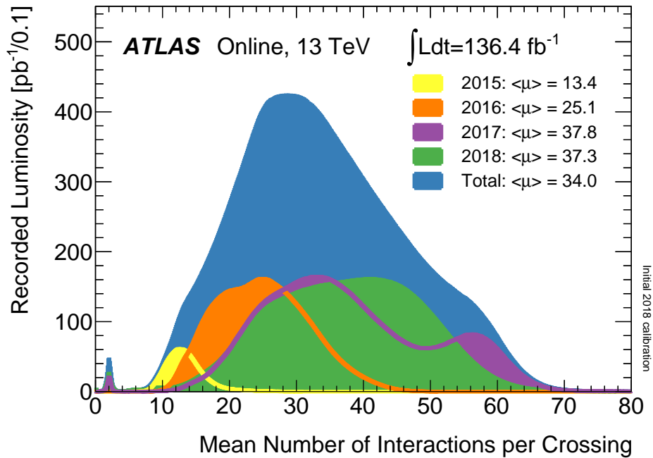
Figure 4.2: The profile of the average number of interactions per bunch crossing at ATLAS is shown for each year of LHC Run 2. Taken from [46].
