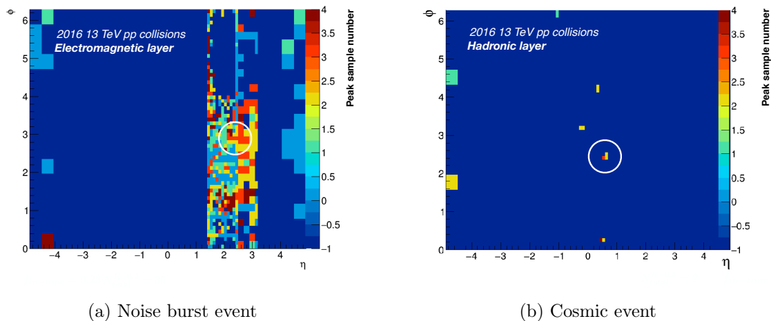
Figure 7.17: An \eta-\phi map of trigger tower channels with pulse activity is shown for (a) a LAr noise burst event and (b) a cosmic ray event. The events were triggered by the Sat80. The peak sample number is shown on the z-axis. Samples are numbered from 1-5, where 3 is the centre sample corresponding to the identified bunch crossing. At the centre of the white circles are saturated trigger tower pulses for which the Sat80 was activated. The number and in-time fraction of trigger towers within the circle is calculated in order to flag possible real mistimed events, as explained in the text.
