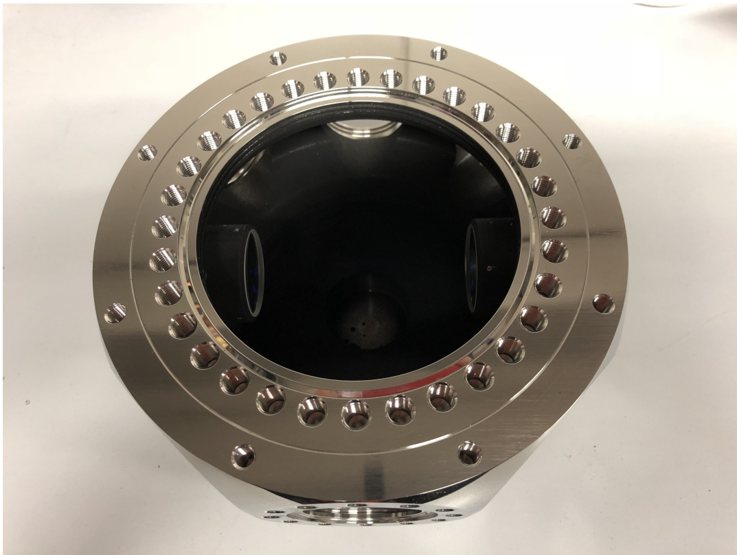
FIGURE 4.25: Coating of the magneto-optical trap and detection optics. The blank stainless-steel surfaces on the inside of the vacuum chamber have been coated with a black paint (AZ Technology MLS-85-SB-C) to reduce stray light. The coating was developed for the use in the Low Earth Orbit space environments and has a low out-gassing rate, therefore suitable for the ultra-high vacuum environment in the magneto-optical trap. The aluminum lens holder tubes have been coated on the outer and inner side. The anti-reflective coated lenses are chosen as large as possible to maximize the numerical aperture and therefore the signal of single atoms.
