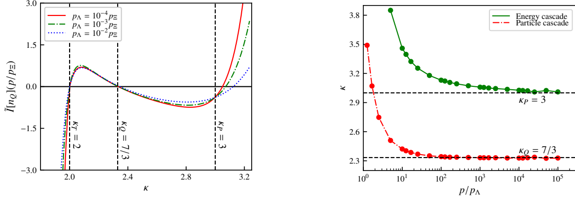
FIG. 6. Left panel: Dependence of the perturbative Boltzmann scattering integral I[n_Q](p) for free particles ( z = 2 , \eta = 0 ; n = n_Q ) in d = 3 spatial dimensions, at the momentum p = 1.5p_E , on the momentum scaling exponent \kappa characterizing the occupation number distribution n(p) \sim p^{-\kappa} . The vertical dashed lines mark, from the left, the thermal zero at \kappa_T = 2 , the particle-cascade exponent \kappa_Q = 7/3 , and the energy-cascade exponent \kappa_P = 3 . In the figure, the rescaled integral \tilde{I}[n_Q](p/p_E) = (2\pi)^3 p_E^{3\kappa-4} (2m g^2 \Lambda^{3\kappa})^{-1} I[n_Q](p) is shown, see Eq. (E.8) for the definition of \Lambda . The different colors (line styles) correspond to different values of the IR cutoff p_\Lambda , as indicated in the legend. As the cutoff is lowered, the zeroes approach the predicted values. The sign of the slope \partial I[n_Q]/\partial \kappa at the zeroes determines the direction of the cascade. Right panel: Scaling exponents \kappa of occupation number distribution n(p) \sim p^{-\kappa} for which the perturbative Boltzmann scattering integral I[n](p) for free particles ( z = 2 , \eta = 0 ; n = n_Q ) in d = 3 spatial dimensions has a zero, for different momenta p in units of the IR cutoff scale p_\Lambda . Lower line: particle cascade for which \kappa approaches \kappa_Q = 7/3 for p_\Lambda \rightarrow 0 . Upper line: zeroes of the energy cascade, approaching \kappa_P = 3 . We emphasize that the two lines represent different physical situations and, as \kappa_Q = 7/3 < d = 3 , due to constraints from conservation laws, only the inverse quasiparticle cascade, is relevant in an isolated system, cf. Sect. II C 1.
