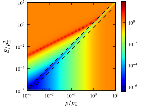
FIG. 5. Contour plot of the effective coupling function g_{\text{eff}}(E, p)/g of free particles, for d = 3 , as a function of E = 2mp^0 and p = |\mathbf{p}| , for p_{\Lambda} = 10^{-3}p_{\pm} . This function enters the T -matrix as defined in Eq. (71). Cuts through this function, for E = 1.5 p^2 and E = 0.5 p^2 (black dashed lines), are shown in Fig. 4. The quasiparticle distribution n_Q was chosen to scale with \kappa = 3.5 . The coupling function in the collective-scattering region (73), is well described by the universal form (74) which does not depend on \kappa . The scattering resonance marked by the dark red ‘ridge’ is centered around the Bogoliubov-type energy-momentum transfer E = [2p_{\pm}^2 p^2 + p^4]^{1/2} .
