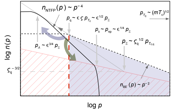
FIG. B.1. Exemplary momentum distribution at a non-thermal fixed point ( n_{\text{NTFP}}(p) , solid line), vs. pre-quench thermal Bose-Einstein distribution in the Rayleigh-Jeans regime, |\mu| \ll k_B T_c (short-dashed line). All particles to the right of the red long-dashed vertical line at p = p_q are removed in the strong cooling quench, p_q < \zeta p_{T_c} (shaded area, see main text). In d = 3 dimensions, according to our kinetic theory, the NTFP distribution of modes with frequency \omega(p) \sim p^2 shows power-law scaling as n_{\text{NTFP}}(p) \sim p^{-4} and evolves self-similarly in time, see Fig. 1(b). The figure shows the special, transient case of such a distribution with a single momentum power law (black solid line). As the evolution conserves the total density \rho = \int_{\mathbf{k}} n(\mathbf{p}) , the point [p_\Lambda(t), n_{\text{NTFP}}(p_\Lambda(t))] moves along the grey fine-dotted arrow n_{\text{NTFP}}(p_\Lambda(t)) \sim p_\Lambda(t)^{-3} . The momentum scale where the pre-quench distribution is cut off in the UV, corresponding approximately to the pre-quench critical temperature, p_{T_c} \sim (mT_c)^{1/2} , is outside the graph's frame. The grey vertical arrows mark the momenta corresponding to the quench scale p_q \sim \epsilon \zeta p_{T_c} , with pre-quench diluteness parameter \zeta and some positive number \epsilon < 1 , the post-quench chemical potential scale p_\Xi = (g\rho_q)^{1/2} = \zeta_q^{1/2} p_{T_{c,q}} , with post-quench diluteness parameter \zeta_q and crit. temperature scale p_{T_{c,q}} , and the IR and UV cutoff scales p_\Lambda \sim \epsilon^{3/4} p_\Xi and p_\lambda \sim \epsilon^{1/4} p_\Xi , at the moment when the scaling function is given by the solid line and still entirely within the non-perturbative regime. The regime where the perturbative wave-Boltzmann equation is applicable ( n(p) \ll (ap)^{-1} , cf. Eq. (B.4)) and [106], is marked by the red dashed area. See Secs. B 2 and B 3 for details.
